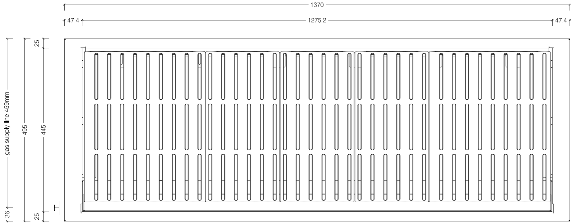
Top View
