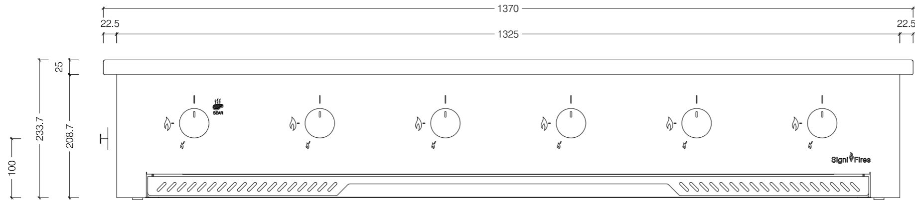
Front View
