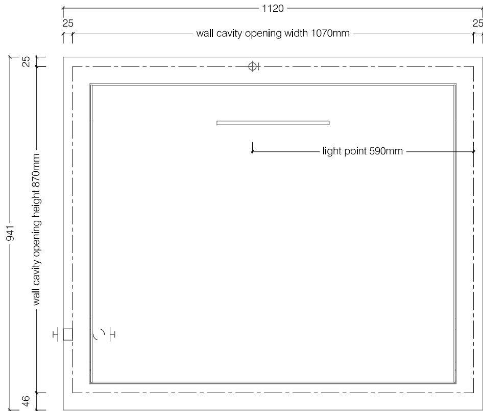
Front View
