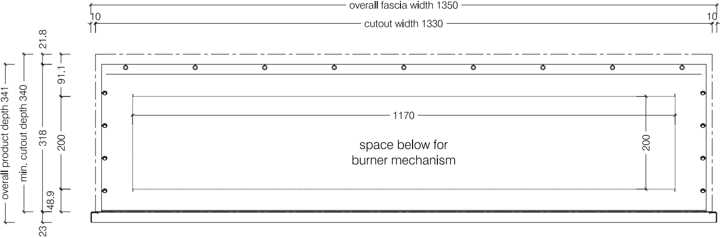
Top View
