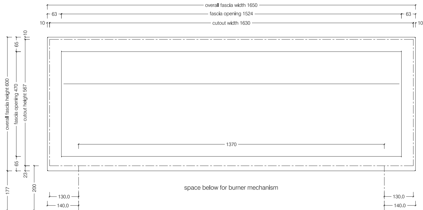
Front View
