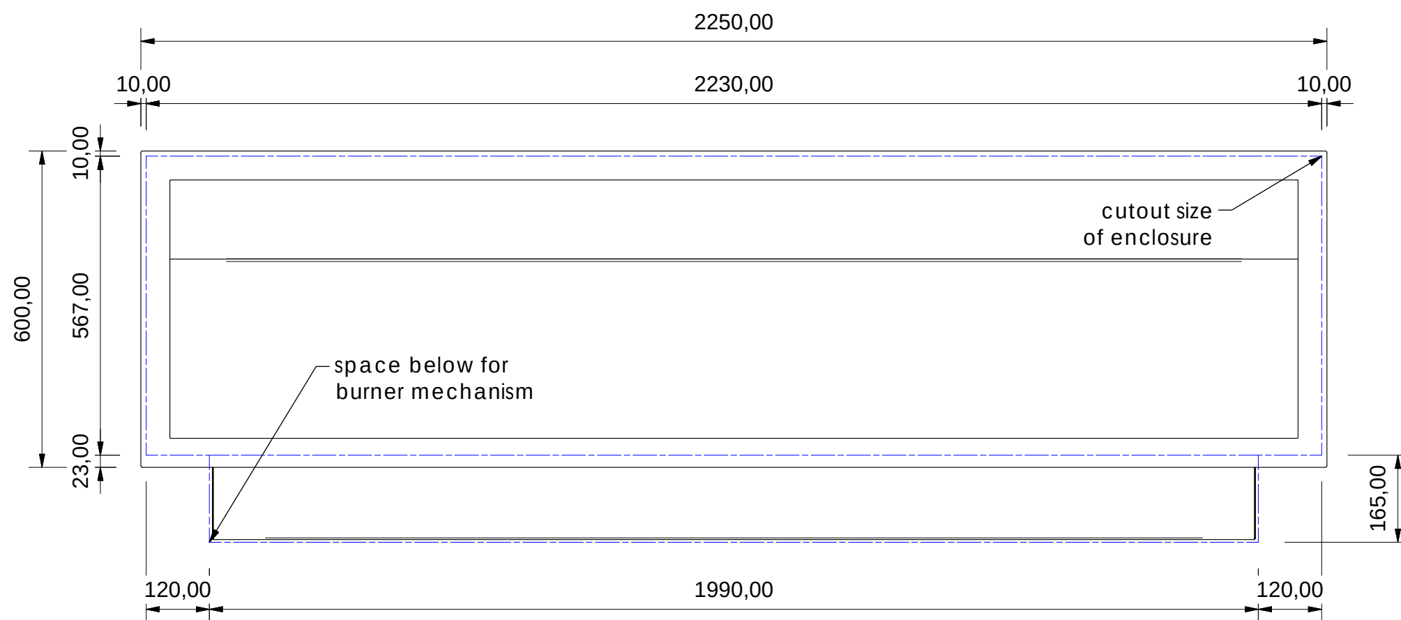
Front View ( 1 : 10 )
