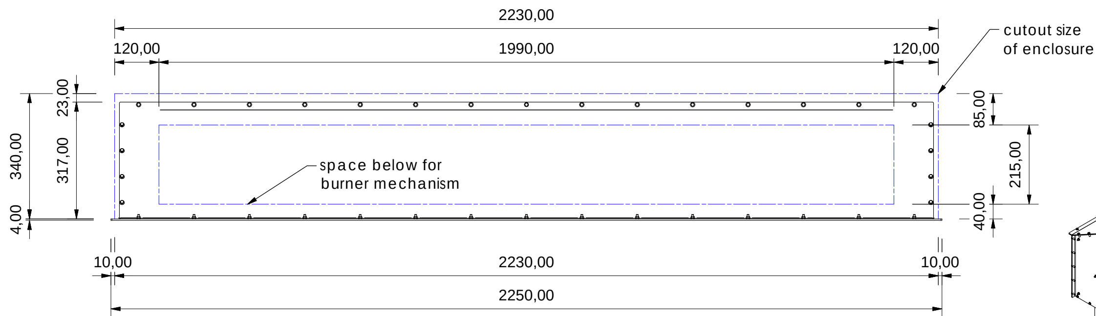
Top View ( 1 : 10 )
